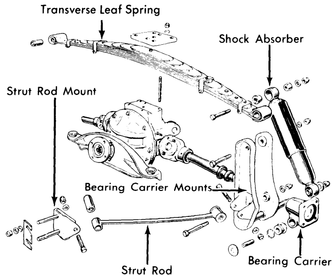
Fig. 1 Exploded View of Rear Suspension Assembly
