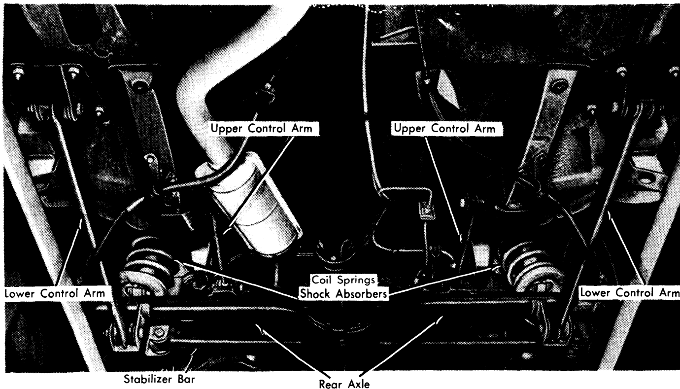
Fig. 1 Installed View of Fiat 124 Rear Suspension Assembly
