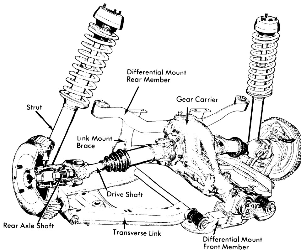
Fig. 1 Datsun 280Z Rear Suspension Assembly
