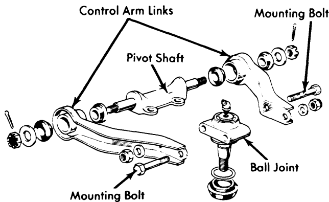
Fig. 3 Exploded View of Upper Control Arm Assembly
