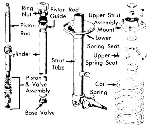
Fig. 2 Exploded View of Corolla Strut Assembly
