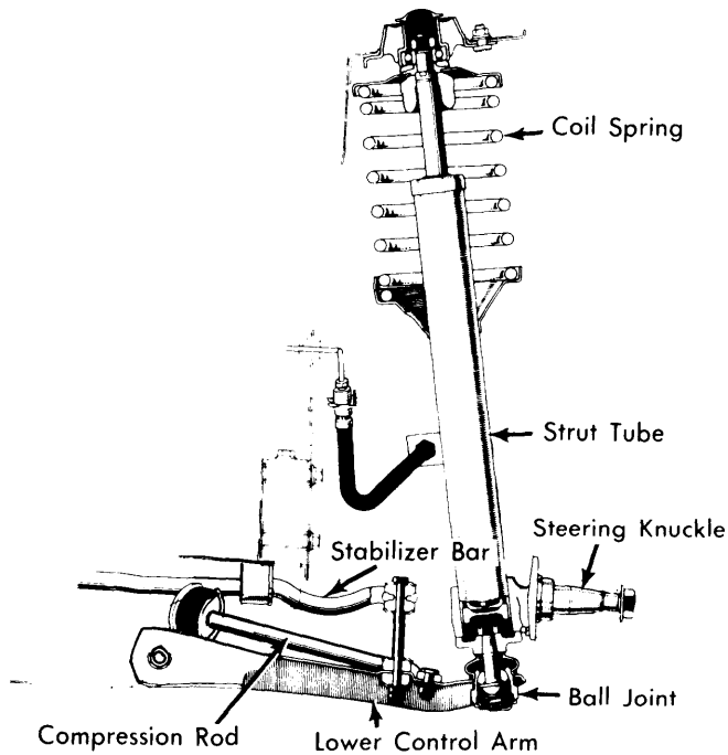
Fig. 1 Celica & Corolla Front Suspension Assembly
