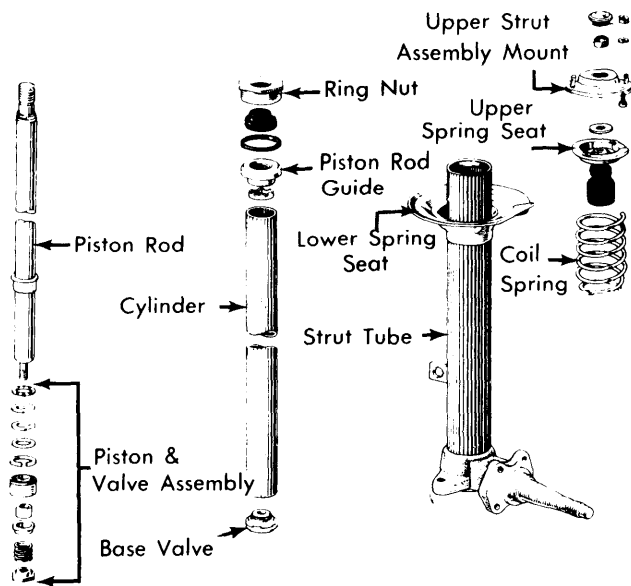
Fig. 3 Exploded View of Celica Strut Assembly
