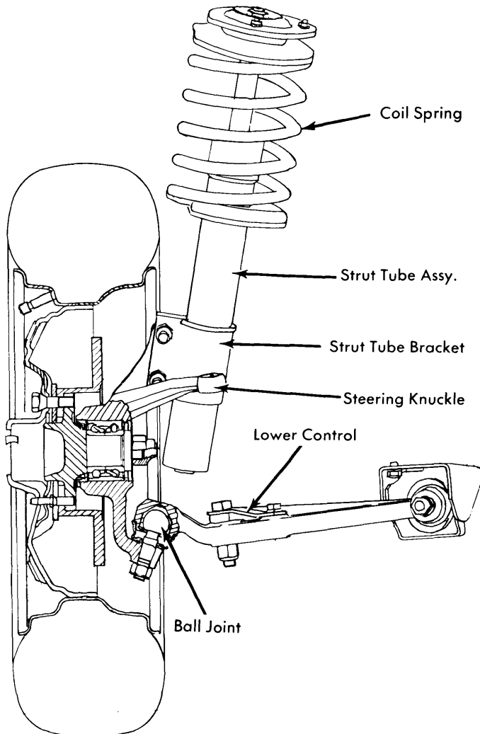
Fig. 1 Sectional View of Front Suspension Assembly
