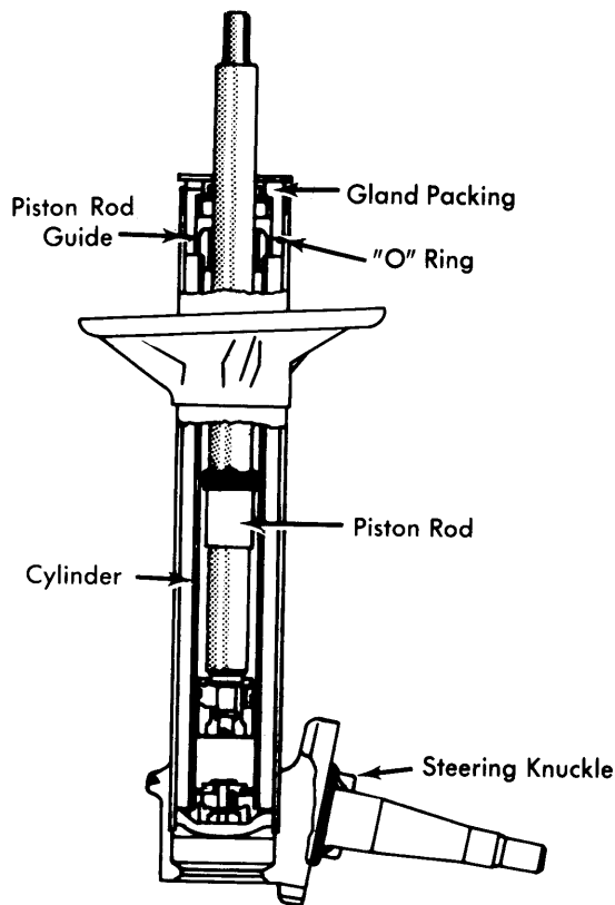
Fig. 2 Sectional View of Suspension Strut Assembly
