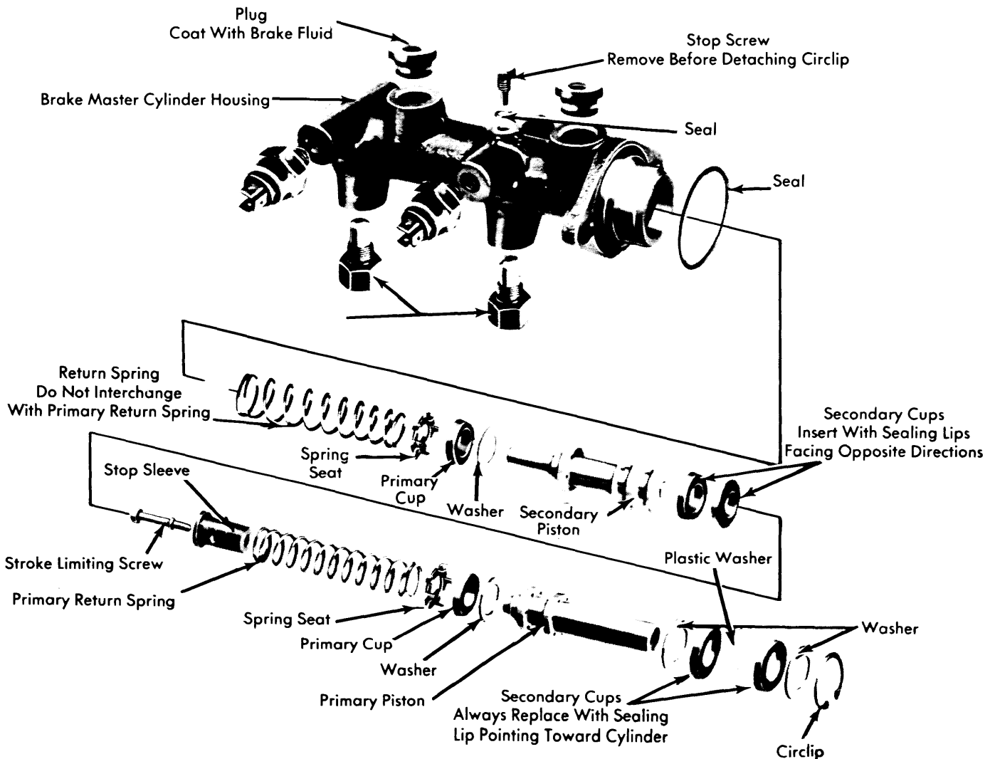
Fig. 7 Master Cylinder Component Relationship — Rabbit, Scirocco, Dasher
