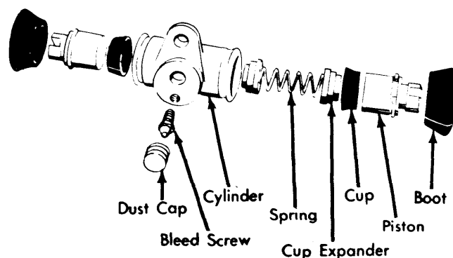
Fig. 6 Volkswagen Type 1 Wheel Cylinder Exploded View
