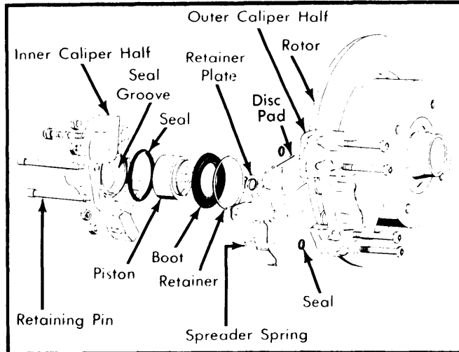
Fig. 2 Disc Brake Assembly Components — Type 2
