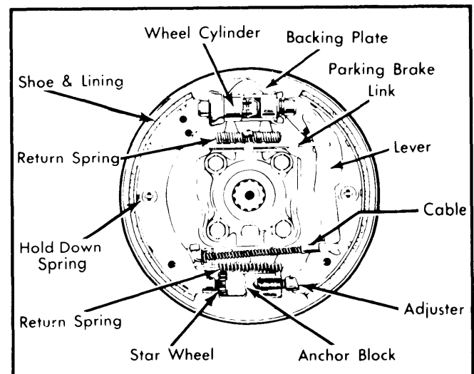
Fig. 4 Volkswagen Type 2 Rear Brake Assembly
