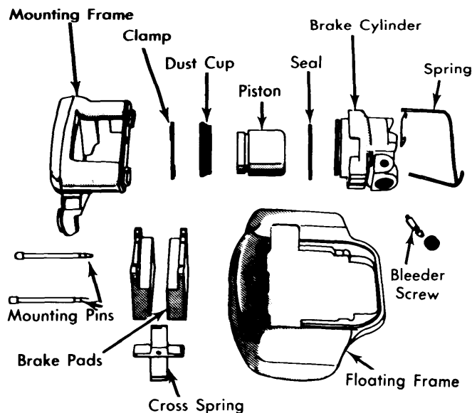
Fig. 5 Disc Brake Caliper Assembly — Dasher, Rabbit, Scirocco
