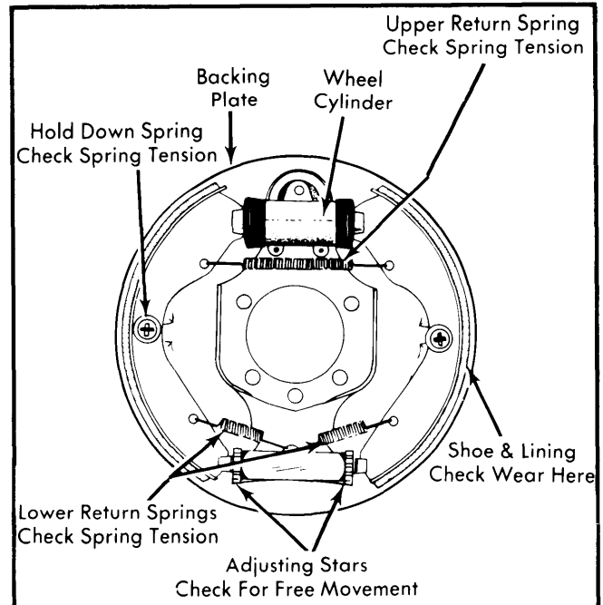
Fig. 3 Volkswagen Type 1 Front Brake Assembly
