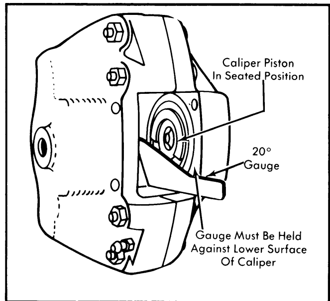
Fig. 1 Using a 20° Gauge to Properly Position Piston
