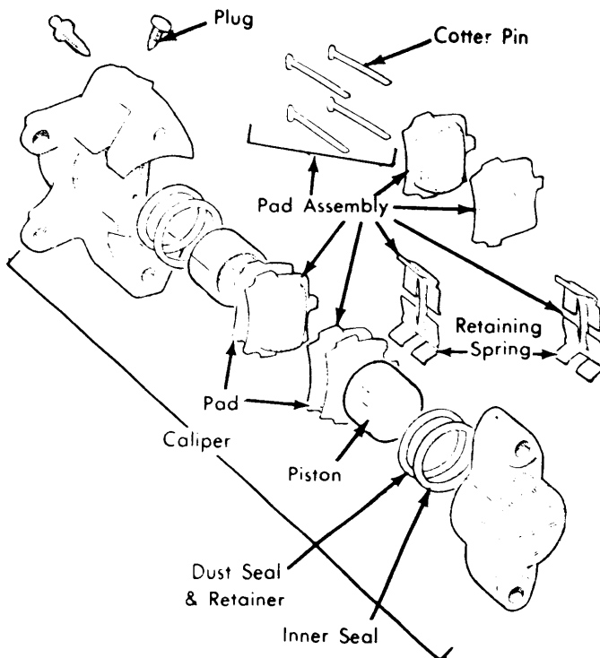
Fig. 2 Exploded View of Front Brake Caliper Assembly
