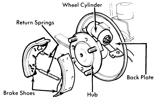
Fig. 1 MG Midget Rear Drum Brake Assembly
