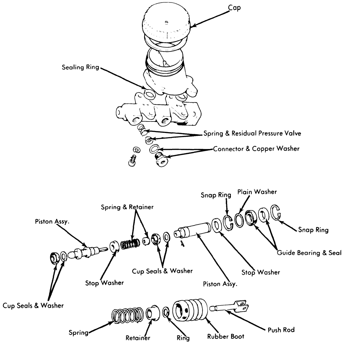
Fig. 4 Master Cylinder Reservoir, Body and Piston Assemblies
