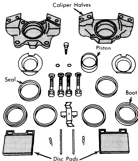
Fig. 5 Disassembled View of Typical Mercedes Benz Brake Caliper
