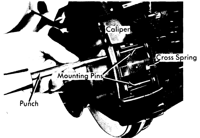
Fig. 2 Knocking Out Disc Pad Mounting Pins On Teves Model Brakes
