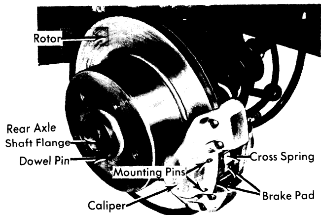
Fig. 4 Assembled View of Rear Hub and Caliper
