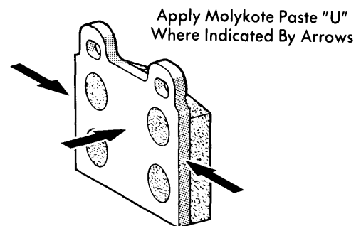
Fig. 3 Typical Mercedes Benz Disc Brake Pad Illustration Shows Molykote Application Points.
