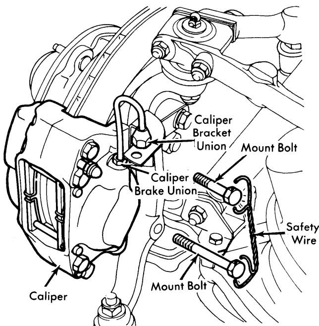
Fig. 4 Assembled View of Disc Brake Caliper with Detail for Removing
