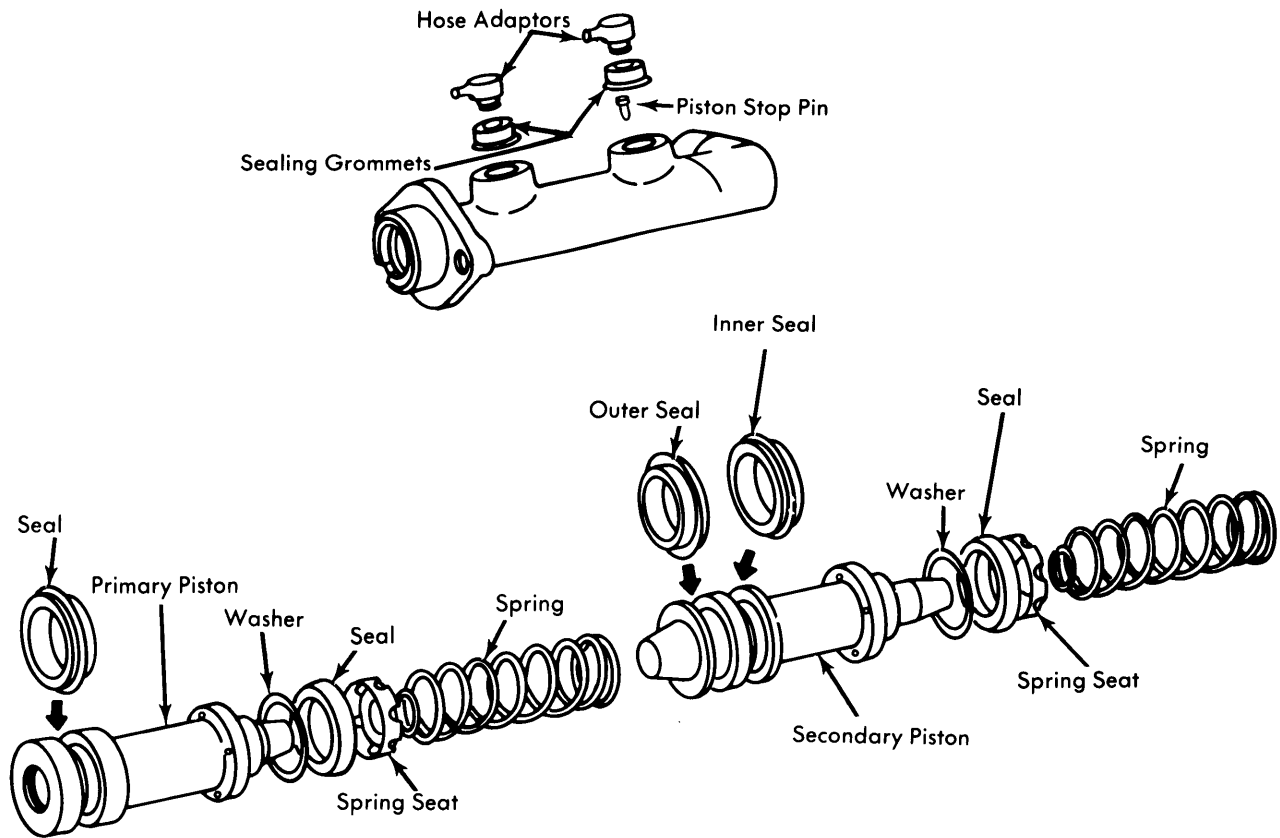
Fig. 6 Exploded View of Jaguar Dual Piston Master Cylinder
