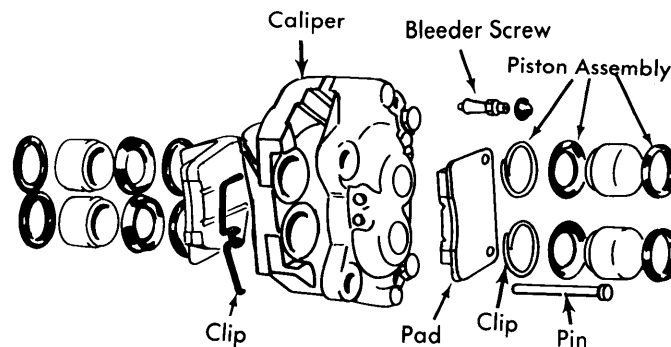
Fig. 2 Expanded View of Front Disc Brake Caliper
