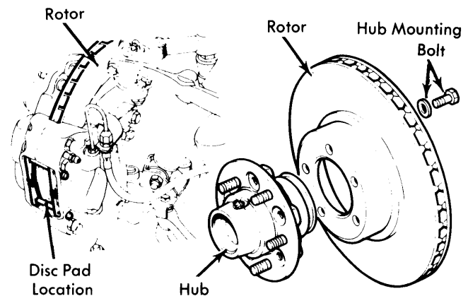
Fig. 5 Assembled View of Rotor and Detail of Hub and Rotor Separation
