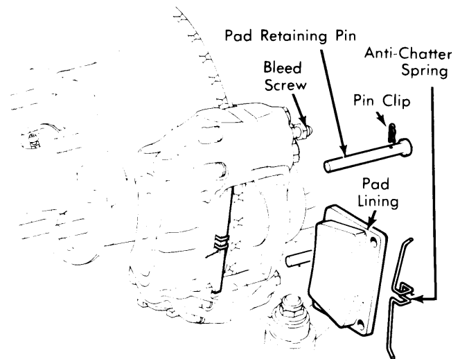
Fig. 1 Front Brake Caliper with Detail of Pad Removal
