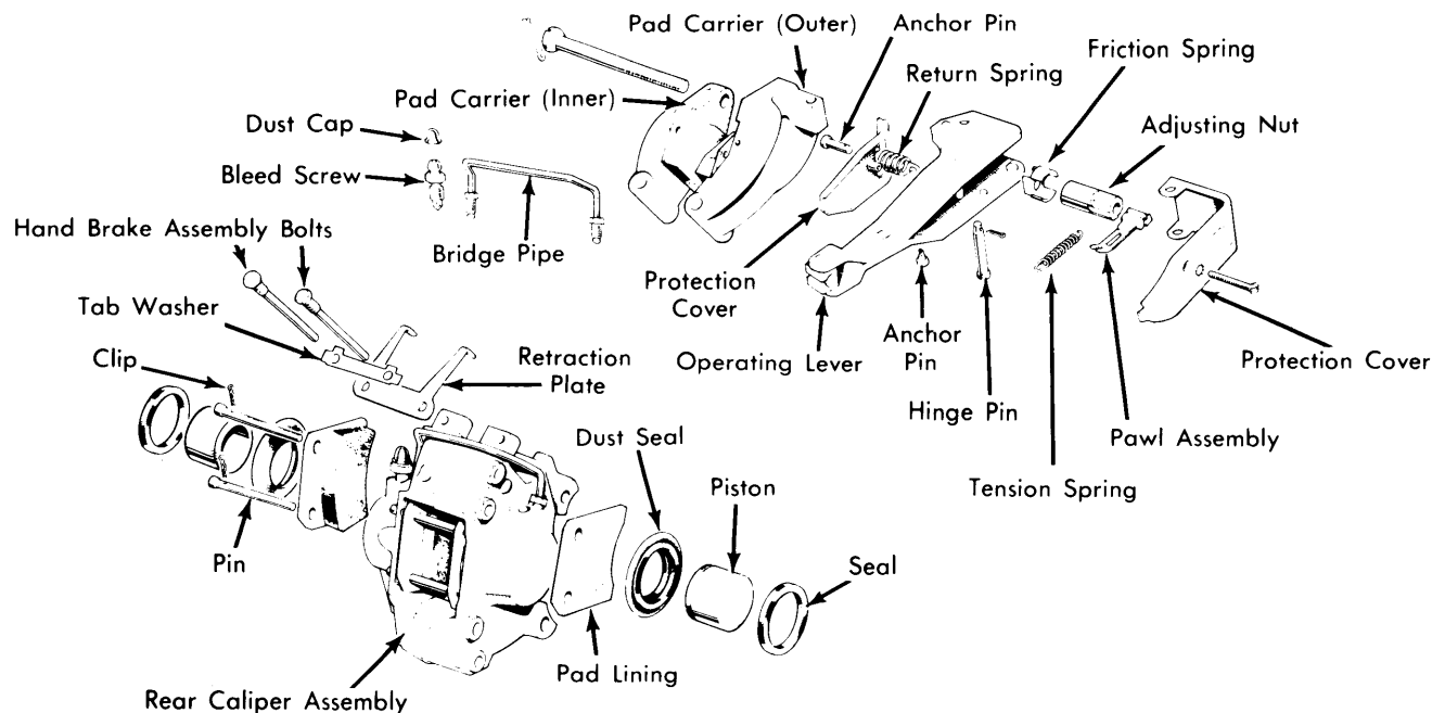
Fig. 3 Exploded View of Rear Disc Brake Caliper with Detail of Parking Brake Assembly
