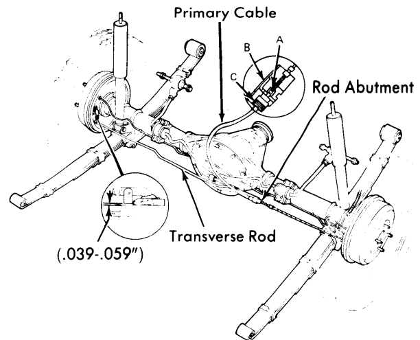
Fig. 1 Parking Brake Adjustment Points
