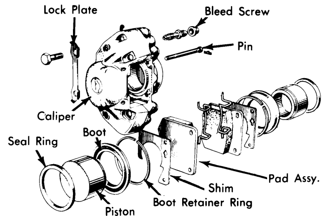
Fig. 2 Exploded View of Front Disc Brake Assembly
