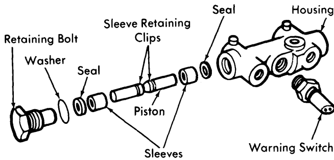
Fig. 6 Pressure Differential Valve Components
