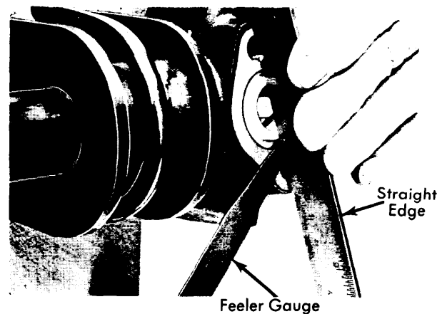
Fig. 1 Measuring Rack Damper Piston End Play
