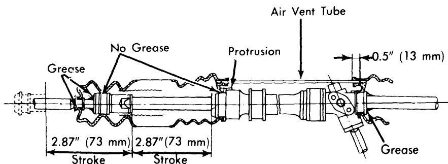
Fig. 3 view Showing Operation Checks and Lubrication of Steering Gear Assembly
