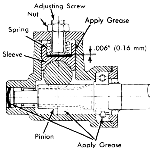
Fig. 4 View Showing Lubrication Points and Backlash Adjustment
