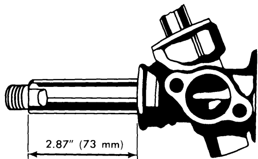
Fig. 2 View Showing Method of Centering Rack in Gear Housing
