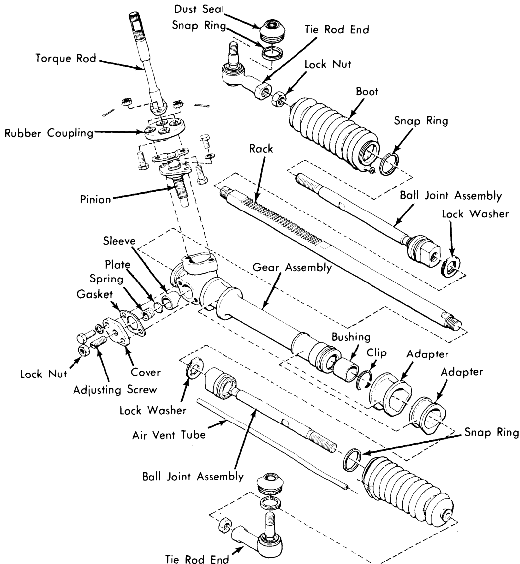
Fig. 1 Exploded View of Subaru Rack and Pinion Steering Gear Assembly
