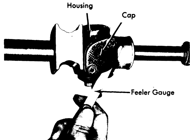
Fig. 4 Measuring Clearance Between Cap and Gear Housing
