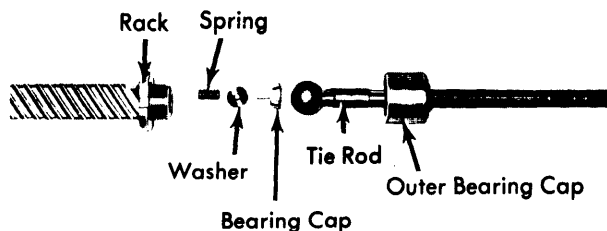
Fig. 3 Exploded View of Ball Joint Assembly Detail
