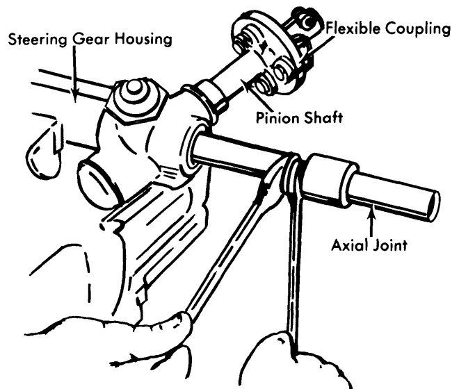
Fig. 2 Separating Axial Joint
