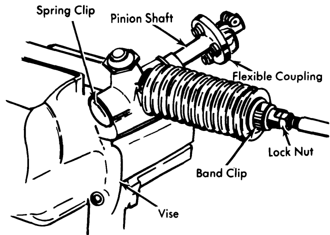
Fig. 1 Removing Tie Rod Ends from Axial Joint
