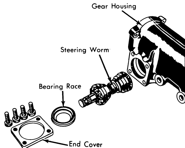
Fig. 6 Steering Worm Shaft and Related Components
