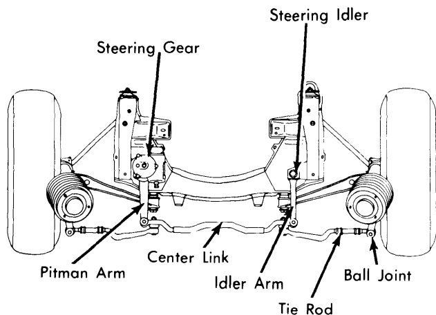
Fig. 1 Top View of BMW Steering Linkage
