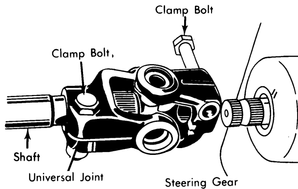
Fig. 3 2002 Lower Universal Joint Coupling at Worm Shaft
