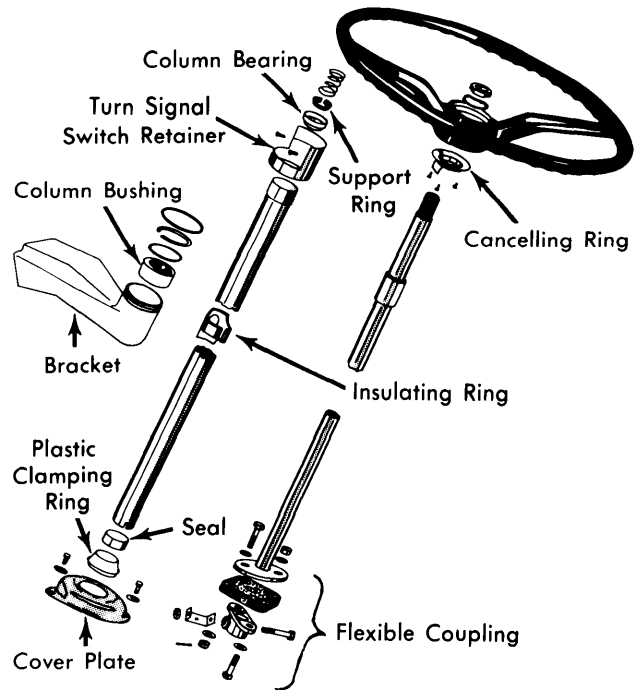
Fig. 1 Type 2 Steering Column and Related Components
