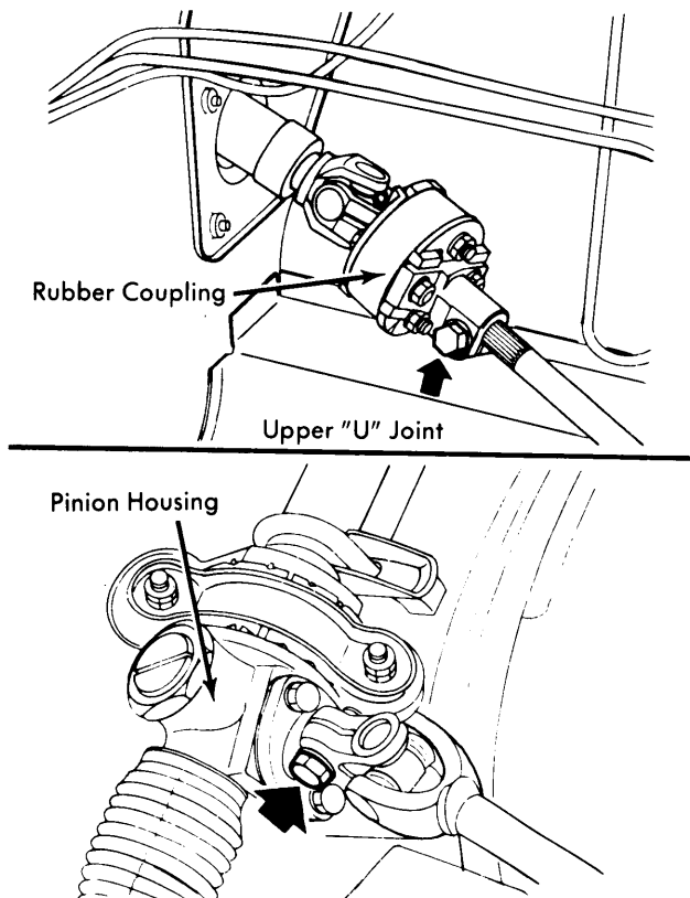
Fig. 1 Details of Steering Column Universal Joints & Couplings
