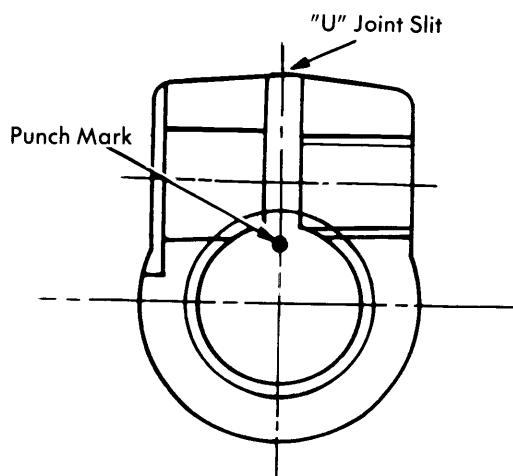
Fig. 2 Detail Showing Punch Mark Alignment
