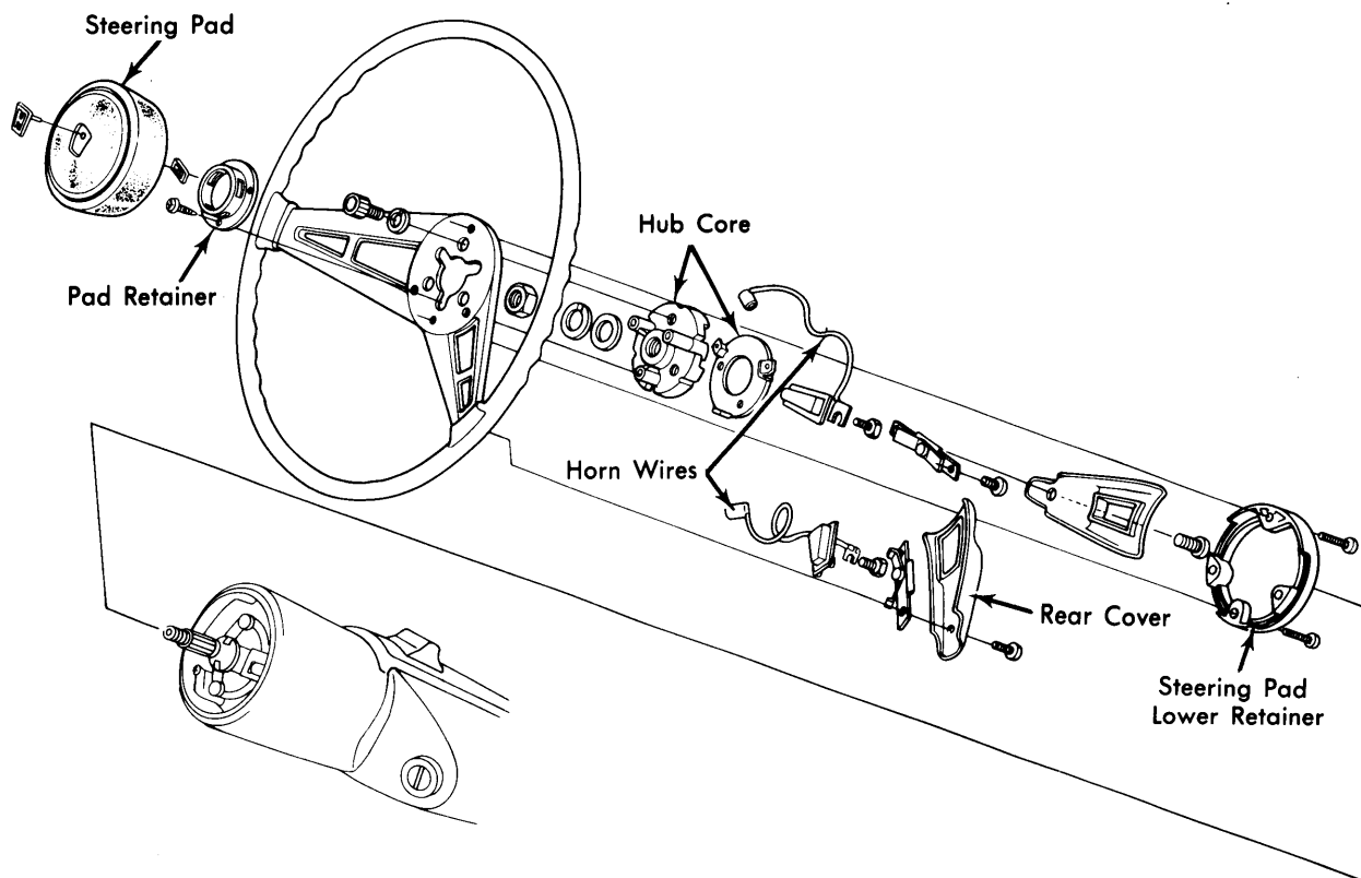
Fig. 1 Exploded View of Honda Steering Wheel with Related Components
