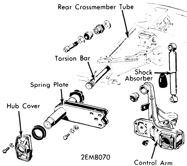
VOLKSWAGEN TYPE 1 REAR SUSPENSION
