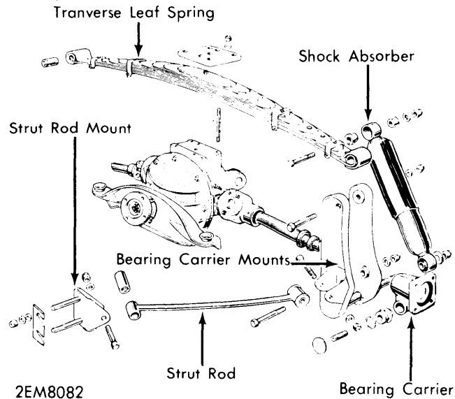
REAR SUSPENSION COMPONENTS
