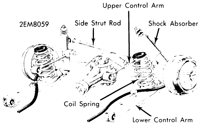
CORONA MARK II REAR SUSPENSION
