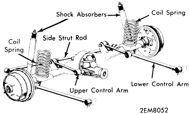
CELICA REAR SUSPENSION COMPONENTS
