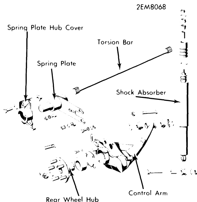
PORSCHE 911 REAR SUSPENSION
