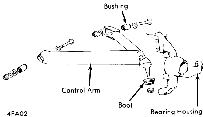
CONTROL ARM ASSEMBLY
