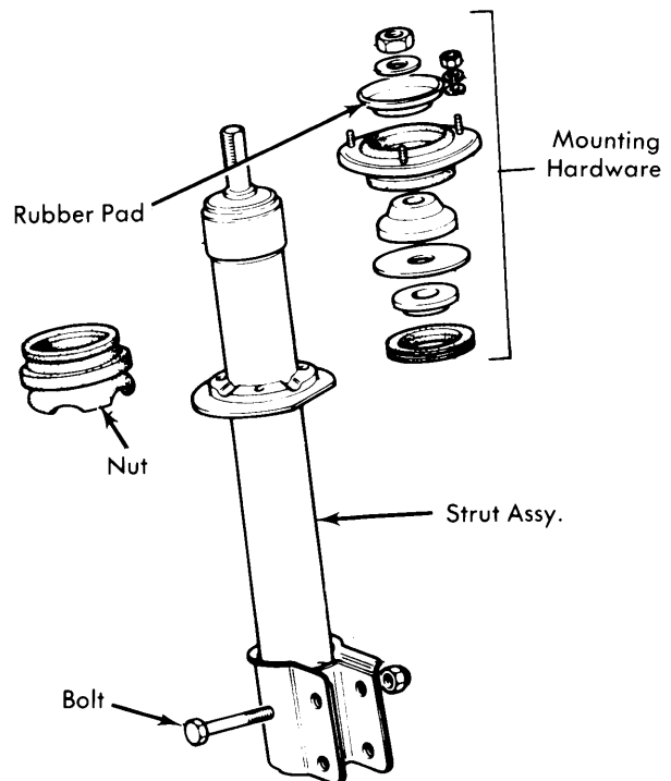
STRUT ASSEMBLY
