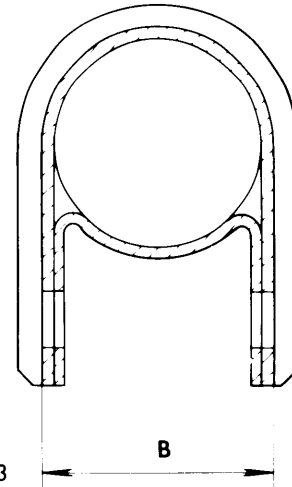
SHIM THICKNESS MEASURING POINT "B"
