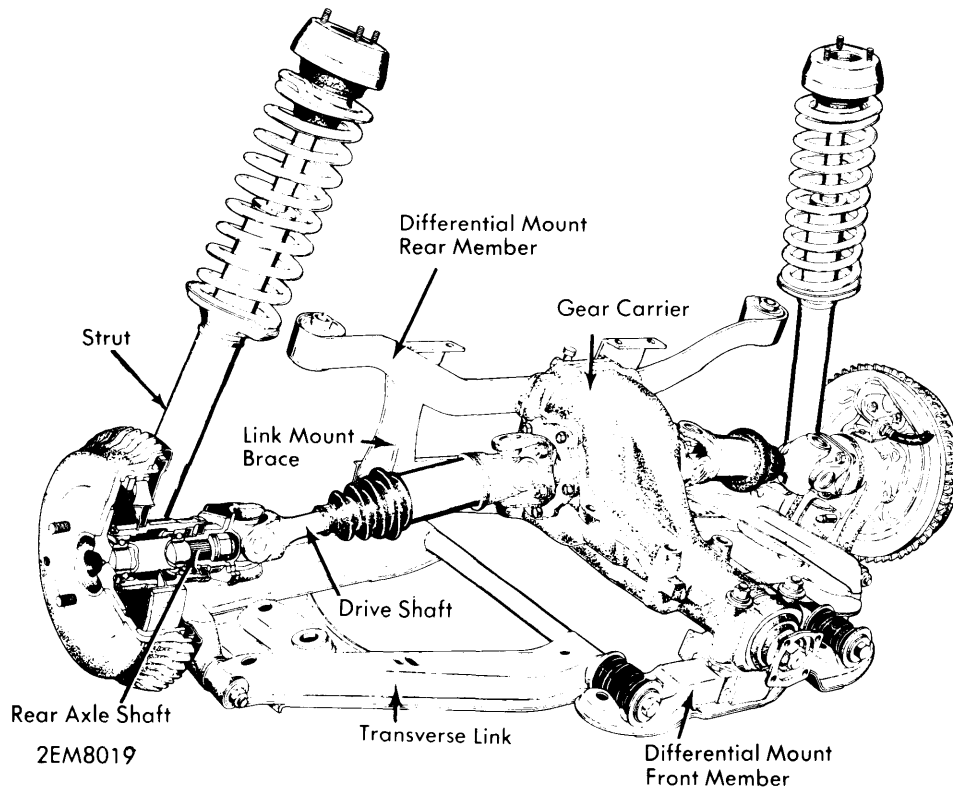
DATSUN 260Z REAR SUSPENSION
