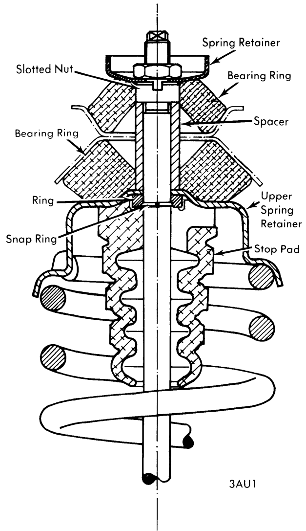
REAR COIL SPRING ASSEMBLY
