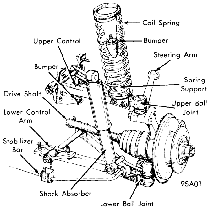
FRONT SUSPENSION COMPONENTS
