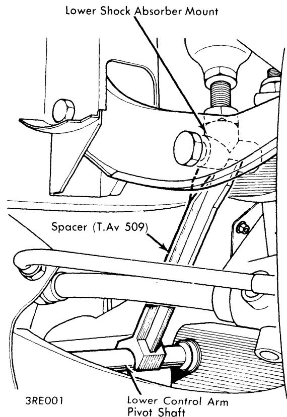
SPACER TOOL INSTALLATION
