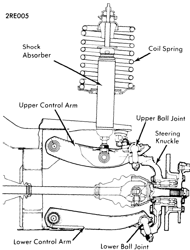
FRONT SUSPENSION ASSEMBLY
