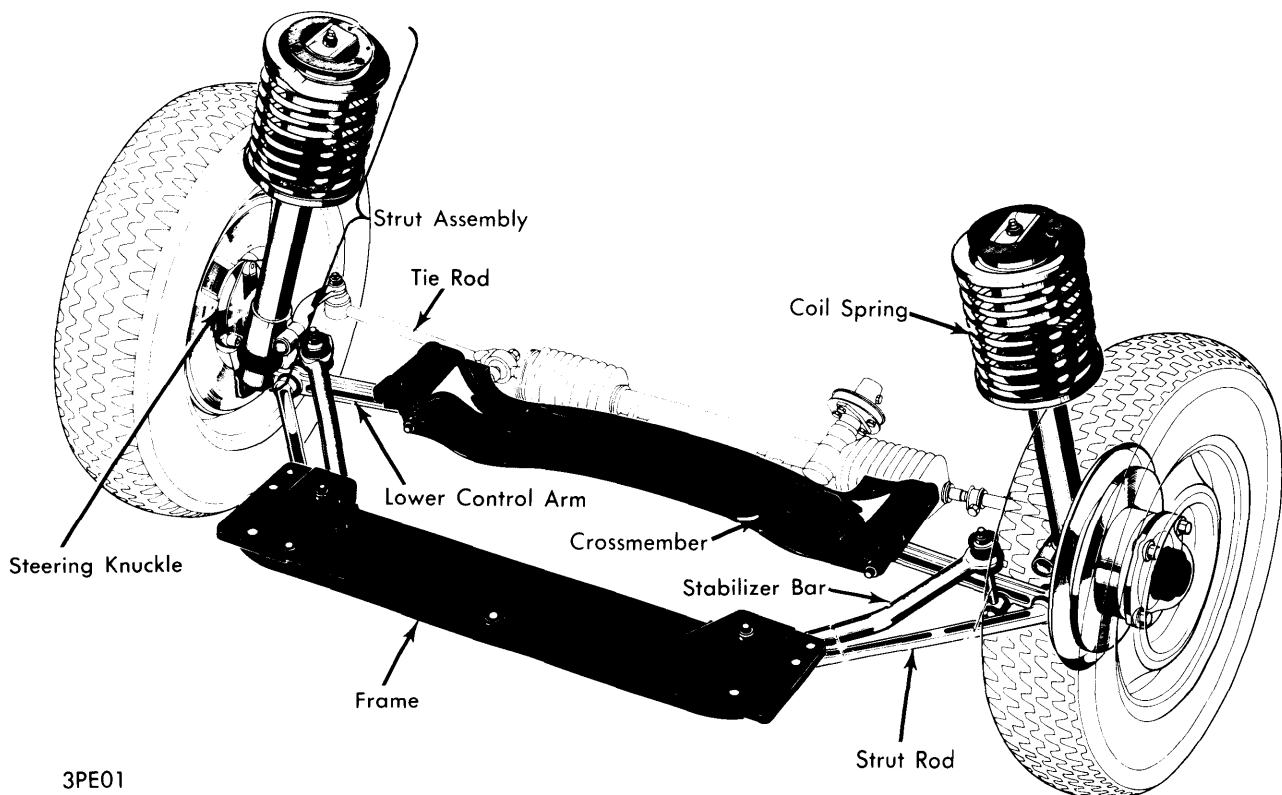
FRONT SUSPENSION ASSEMBLY
