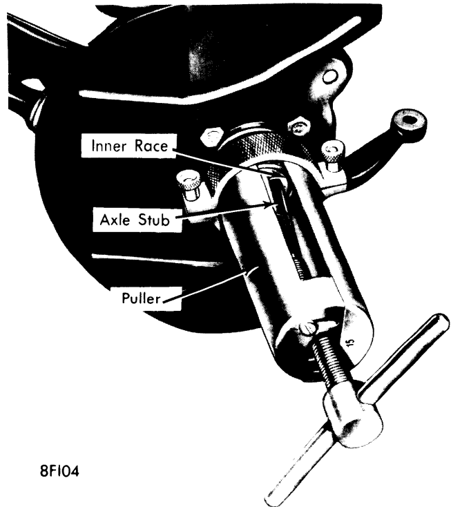
REMOVING INNER RACE FROM INSIDE WHEEL BEARING
