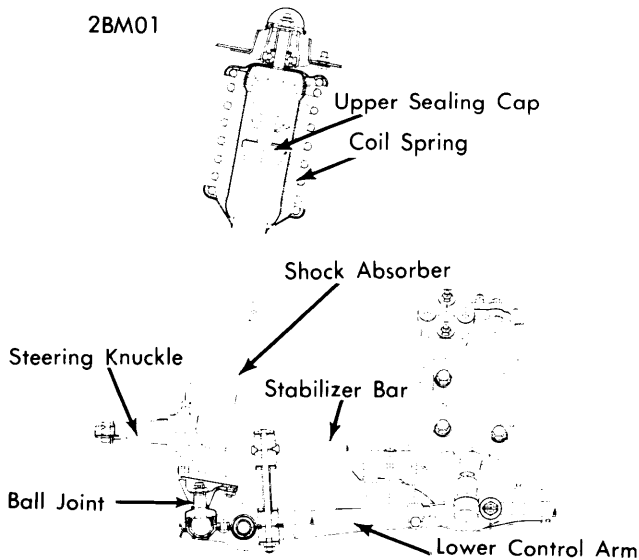
FRONT SUSPENSION ASSEMBLY (TYPICAL)
