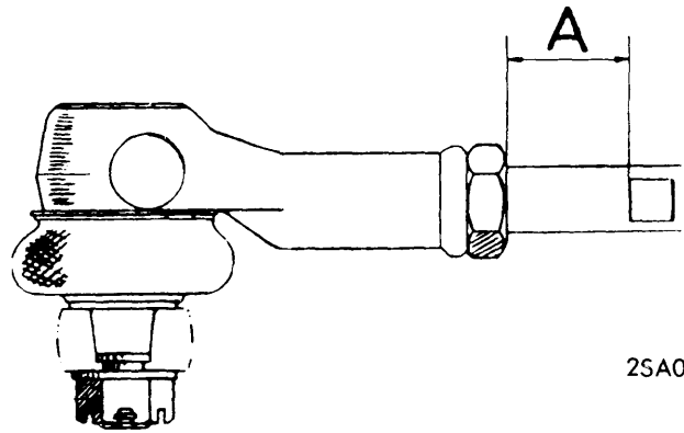
CHECKING LENGTH OF TIE ROD WITH KEY GRIP
