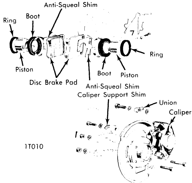
DUAL PISTON CALIPER ASSEMBLY
