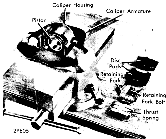
DISASSEMBLING CALIPER ASSEMBLY
