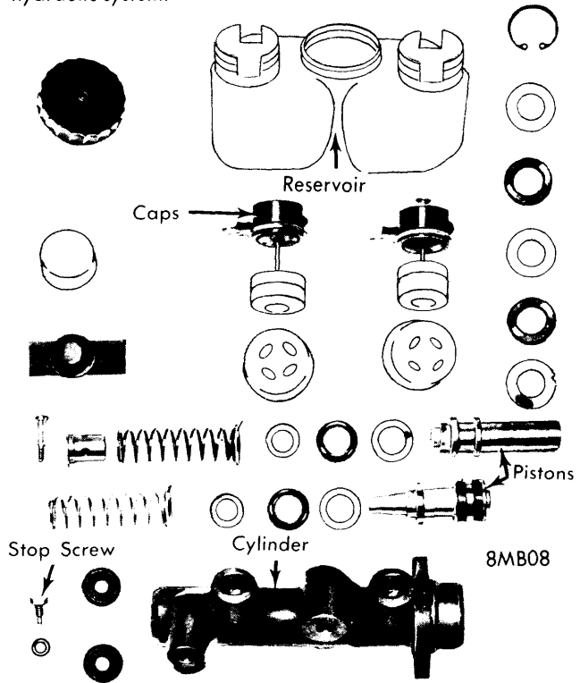
MASTER CYLINDER ASSEMBLY
