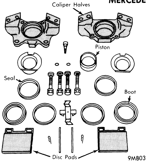
DISC BRAKE CALIPER ASSEMBLY
