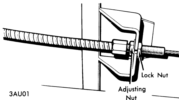
PARKING BRAKE ADJUSTMENT
