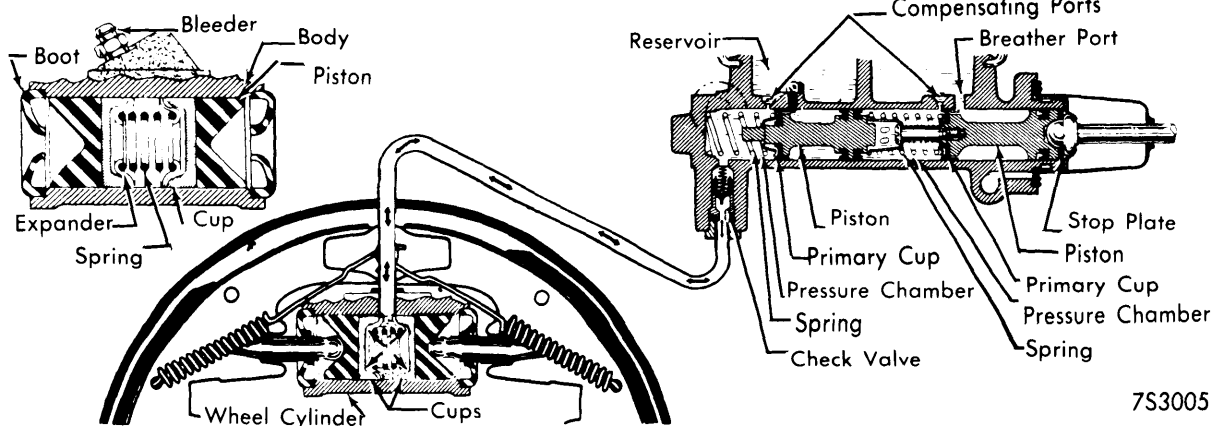
HYDRAULIC BRAKE SYSTEM (TYPICAL)
