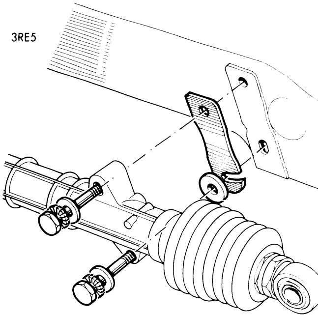
LOCATION OF MOUNTING SHIMS
