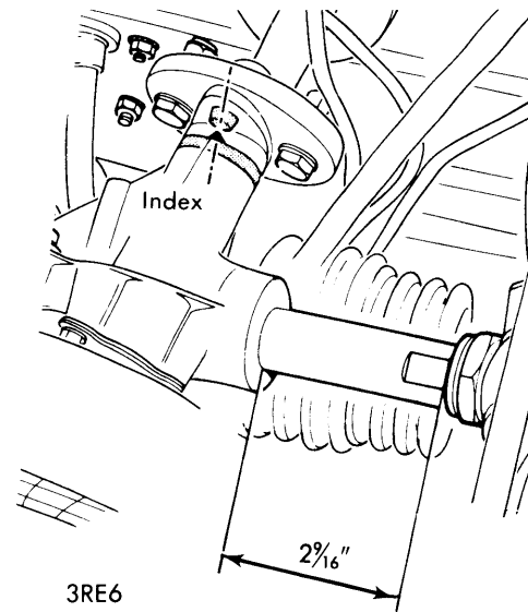
SETTING CENTER POINT
