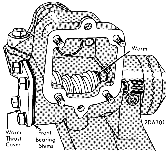
FITTING WORM THRUST COVER
