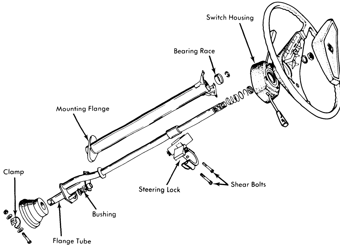
DASHER STEERING COLUMN COMPONENTS
