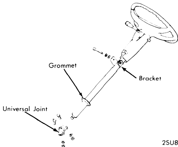
STEERING COLUMN ASSEMBLY
