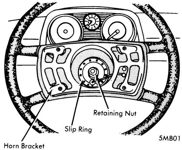
STEERING WHEEL REMOVAL
