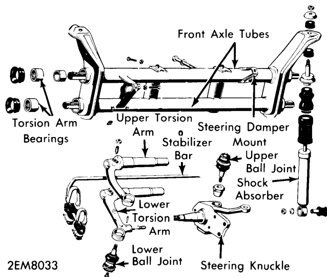
VOLKSWAGEN SEDAN FRONT SUSPENSION COMPONENTS
