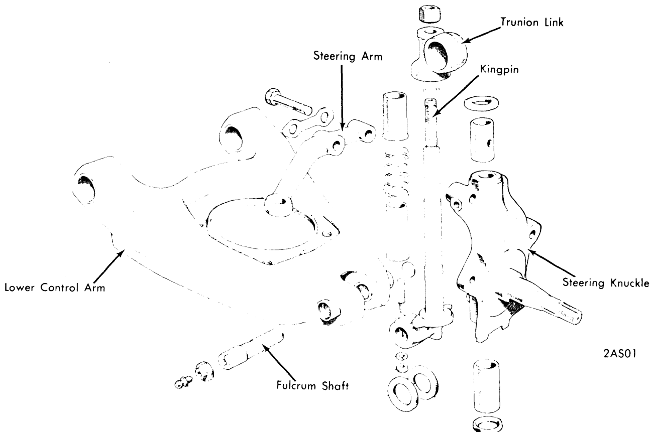
FRONT SUSPENSION COMPONENTS
