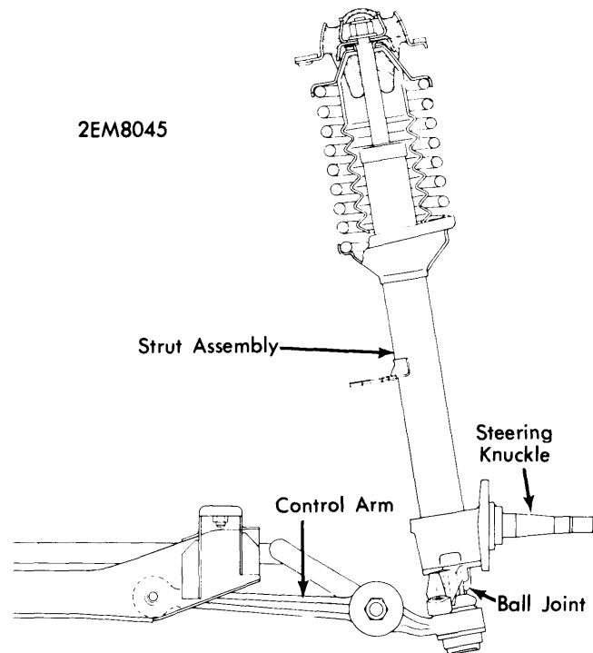
MAZDA 616, RX2 & RX3 FRONT SUSPENSION (TYPICAL)
