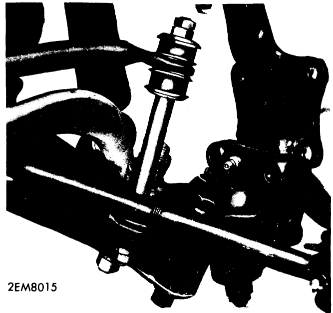
STABILIZER LINK BOLT COMPONENT ARRANGEMENT
