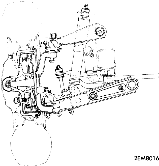
LUV FRONT SUSPENSION
