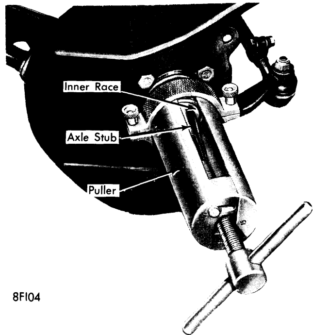
REMOVING INNER RACE FROM INSIDE WHEEL BEARING
