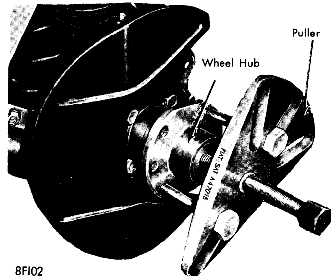
REMOVING FRONT WHEEL HUB
