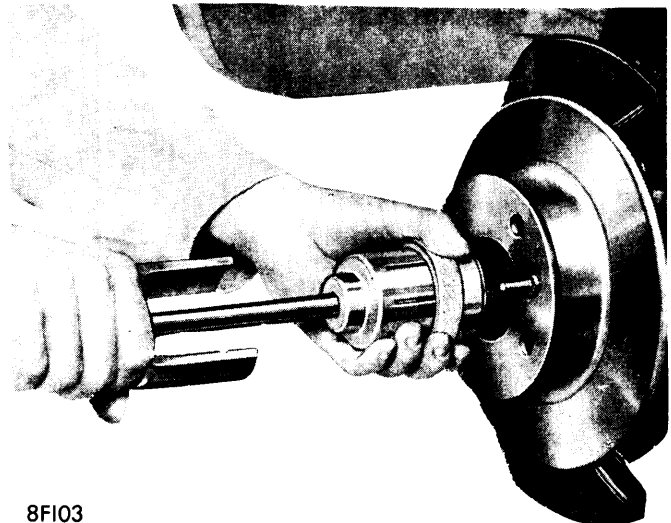
REMOVING FRONT WHEEL HUB CAP
