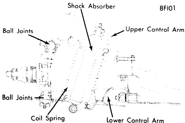
FRONT SUSPENSION ASSEMBLY
